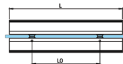
HY2-022 DOOR HANDLE L0:160 L:300 mm HY2-023 DOOR HANDLE L0:30 L:50 mm Hole diameter 9 mm, 6-8-10 mm glass (Brass) (L0:X L:X mm) Made in all sizes
