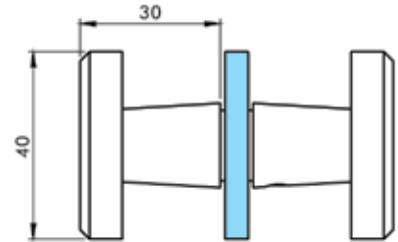
HY2-001 DOOR HANDLE SQUARE Hole diameter 10 mm, 6-8-10 mm gross (Brass)
