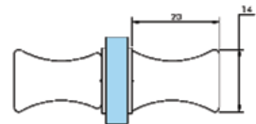
HY2-020 DOOR HANDLE L0:160 L:300 mm HY2-021 DOOR HANDLE L0:30 L:50 mm Hole diameter 9 mm, 6-8-10 mm glass (Aluminium) (L0:X L:X mm) Made in all sizes
